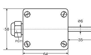
Mounting flange for KF21/31
