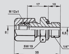
MAU 8 / Nst all dimensions in mm
